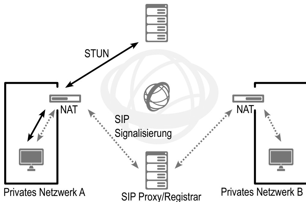
Abb. 16-2: STUN
