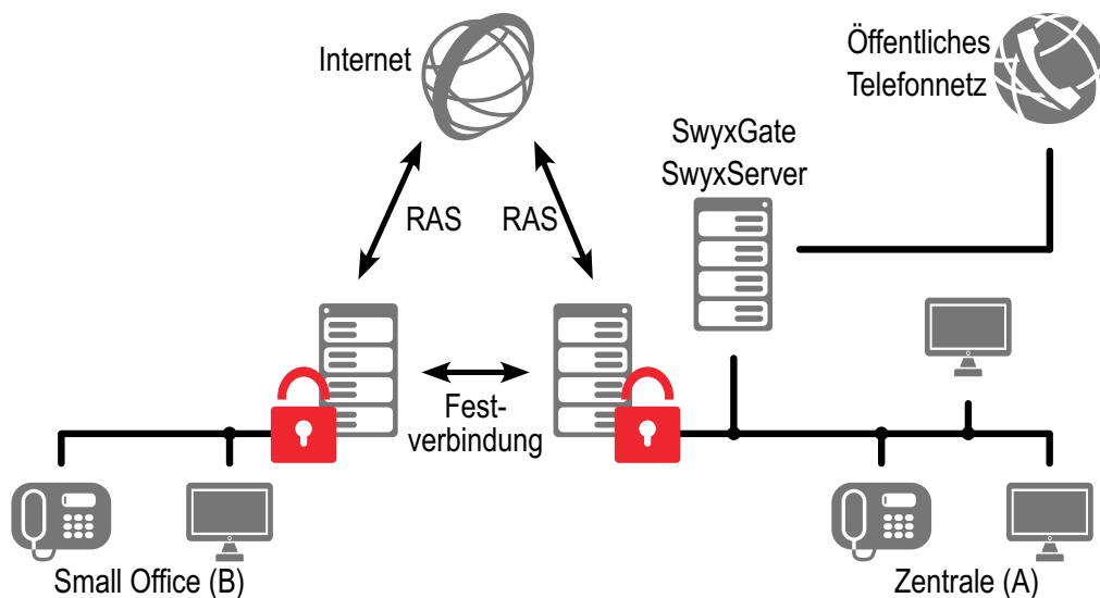
Abb. 26-3: Standortkopplung Small Office
