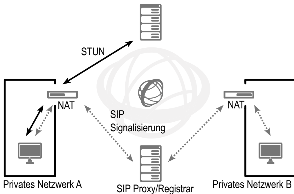
Abb. 16-3: SIP/STUN
